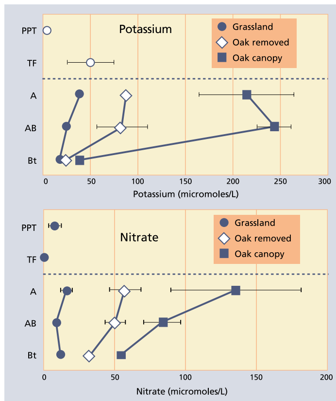
Fig. 3. Concentrations (mean ± standard deviation) of potassium and nitrate in precipitation (PPT), canopy throughfall (TF) and soil solutions from A, AB and Bt horizons of soils at SFREC. Soil solutions were collected from soils beneath the oak canopy, from adjacent grasslands and from sites where blue oaks were removed. Solutions were collected monthly from December through May following removal of the oak trees the previous September.
