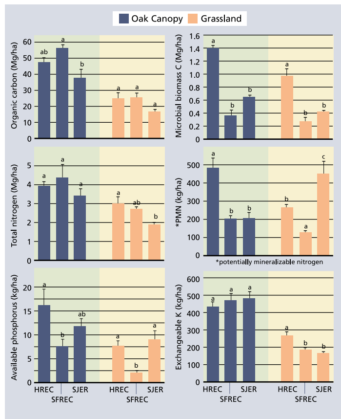
Fig. 2. Organic carbon and nutrient pools (mean ± standard error; n = 5) for the 0-6-inch- (0-15 cm-) depth increment of soils beneath the oak canopy and adjacent grasslands for sites at HREC (sandstone/shale), SFREC (greenstone) and SJER (granite). Means with same lower case letters within each vegetation type (oak versus grassland) are not statistically different at P = 0.05.
