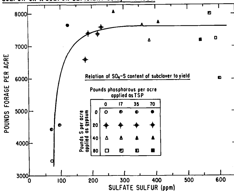
Relation of total forage production to the sulfate sulfur content of subterranean clover plants receiving increasing amounts of sulfur on a sulfur deficient soil.
