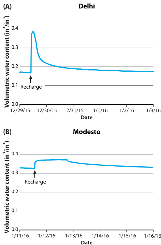
FIG. 2. Volumetric water content (VWC, \text{in}^3/\text{in}^3 ) for winter-watered almond orchards at (A) Delhi and (B) Modesto, measured at 0.5 ft (15 cm; blue solid lines), 1.5 ft (45 cm; black dashed lines) and 3.3 ft (100 cm; red solid lines). Blue bars represent the daily precipitation amount (inches/hour); green bars represent groundwater recharge events.
