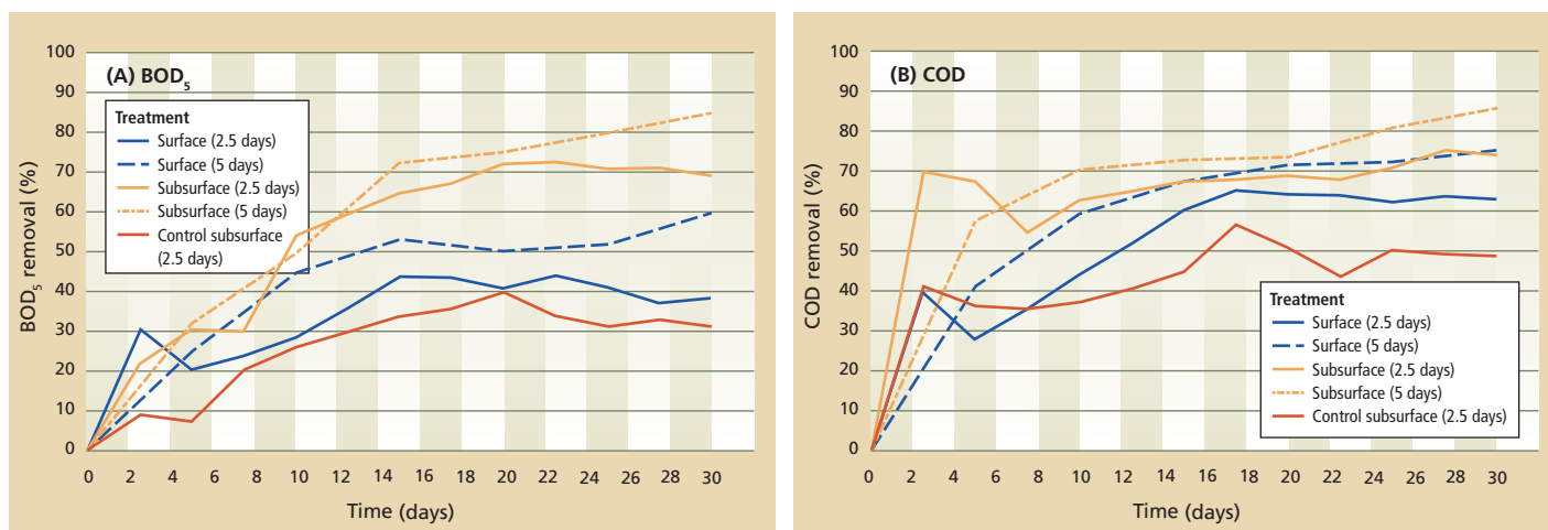
Fig. 2. Daily variation of removal efficiencies for (A) biological oxygen demand, 5 days (BOD 5 ) and (B) chemical oxygen demand (COD) in constructed-wetland greenhouse flume experiments.
