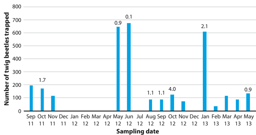
FIG. 3. The number of twig beetles recovered from traps baited with the pheromone pitonyl on the dates (month/year) indicated. The height of each bar represents the total for traps placed at six locations in the Monterey pine forest. The number above the bar is the percentage of beetles from which Fusarium circinatum was isolated. The absence of a number indicates that the pathogen was not recovered from any twig beetles on that date.
