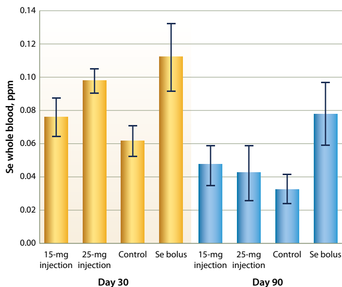
Fig. 1. Se whole blood levels (ppm) with 95% confidence intervals based on treatment and sample date for trial 1, 2011.
