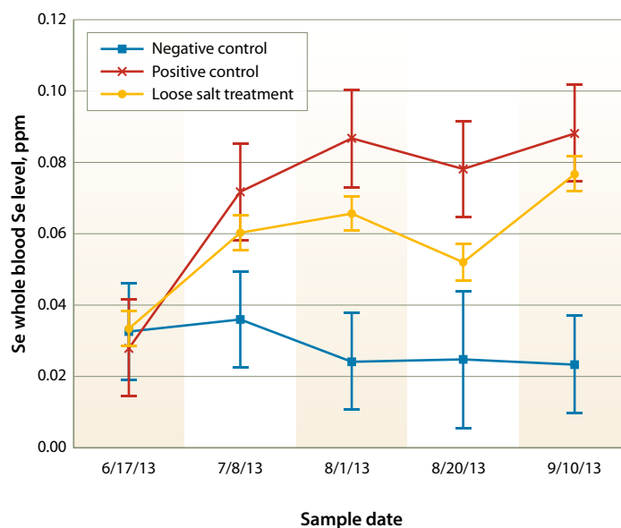
Fig. 2. Whole blood Se response with least significant differences by treatment and date in trial 2, 2013.
